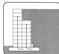
VERTICAL R.C. FILLED WALL
